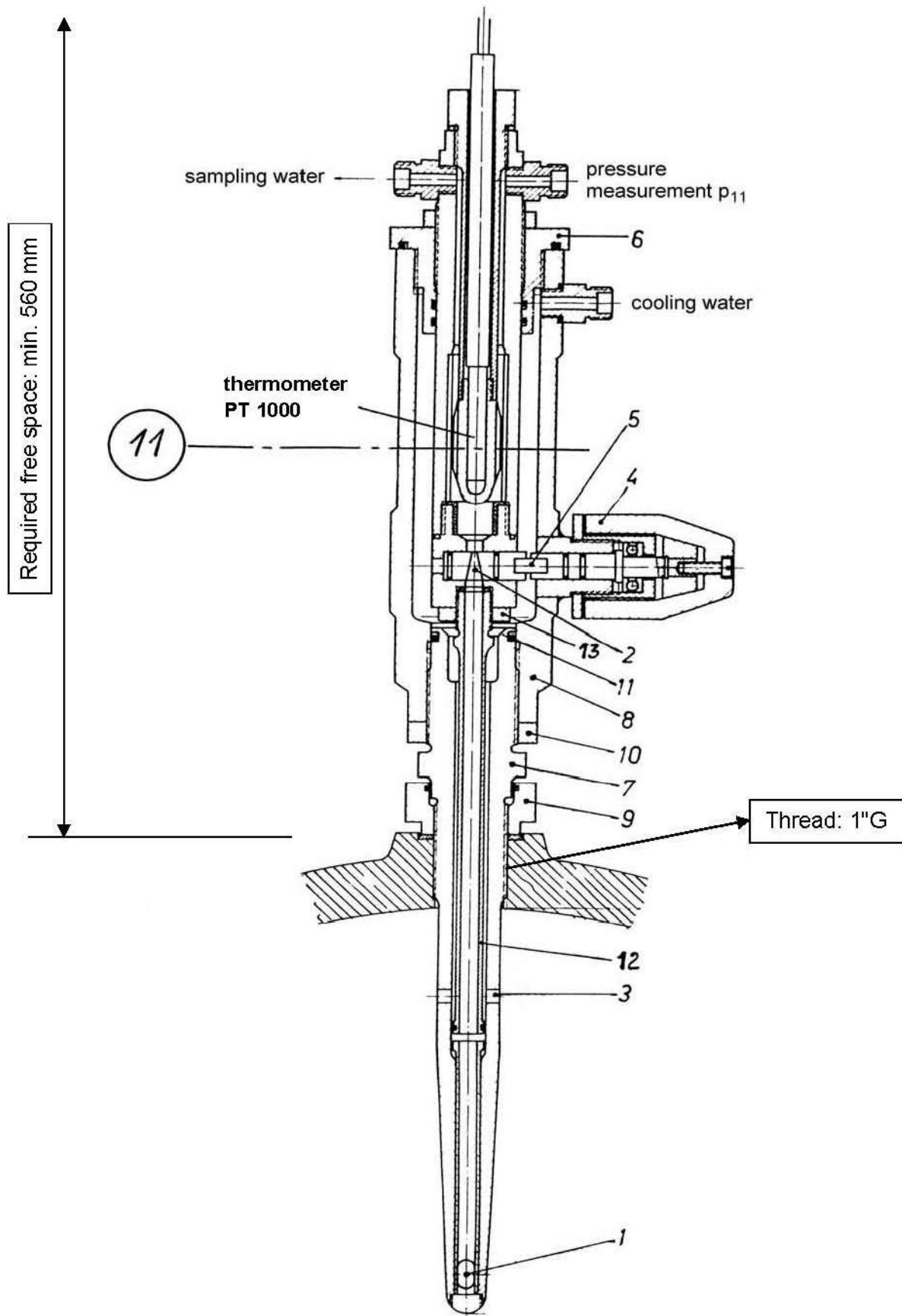
Sampling probe with adjustable expanding device
