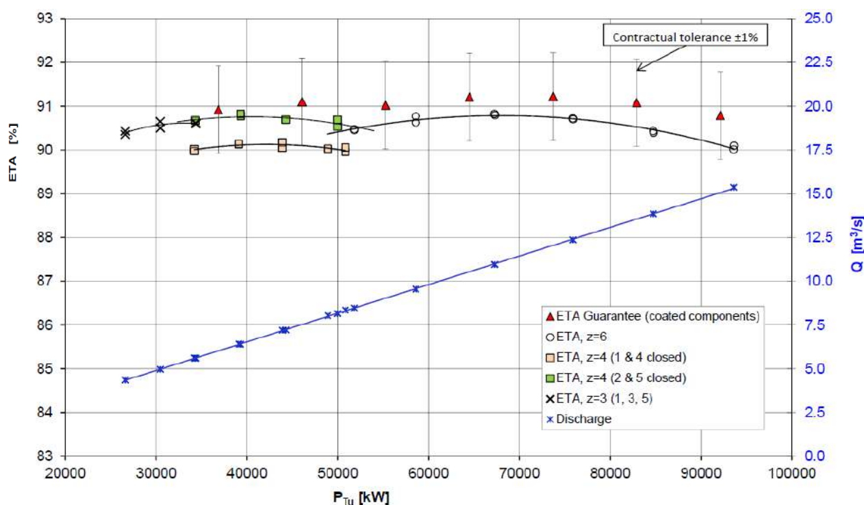
Figure 2: Results converted to rated head
