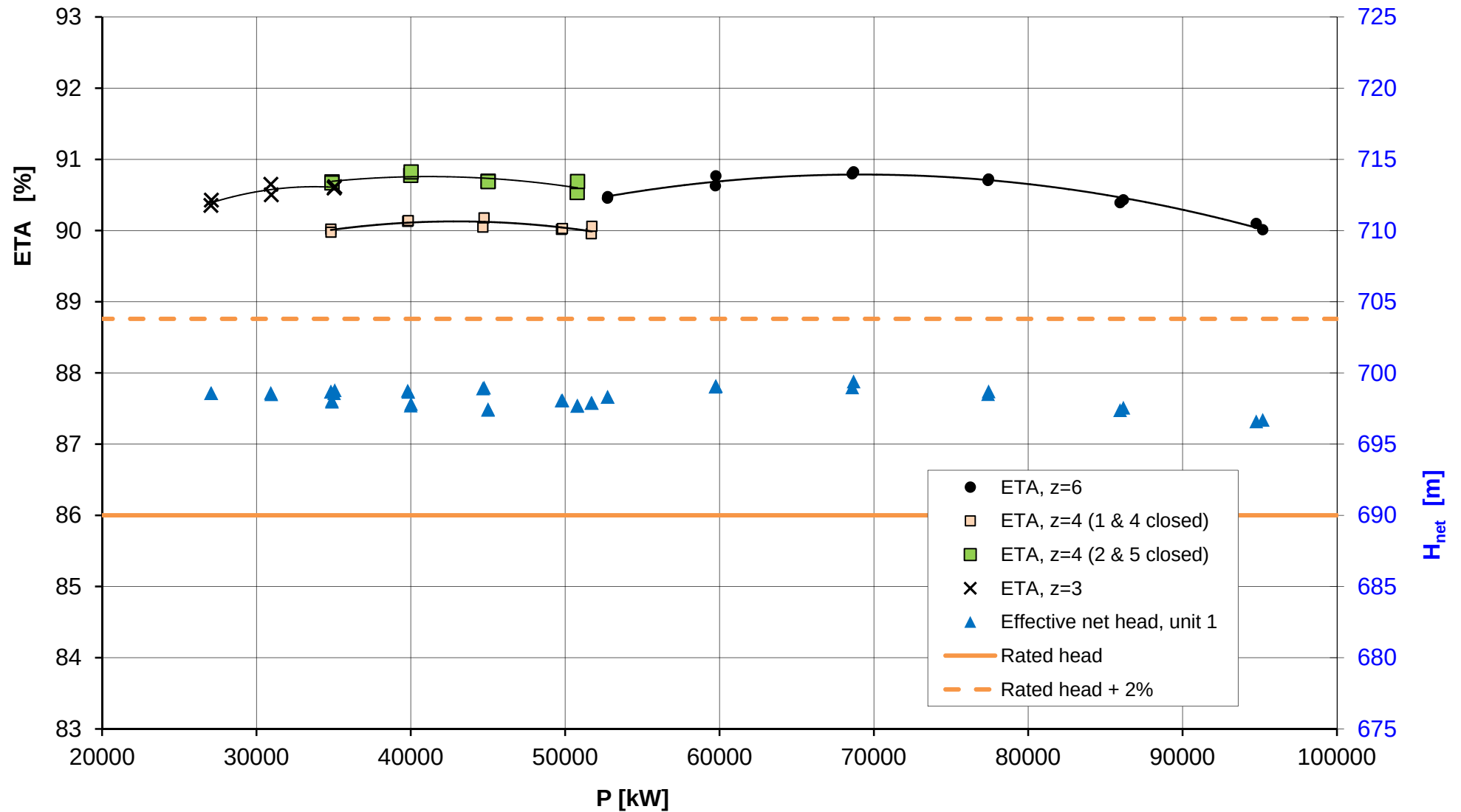
Resultats at measured net head
