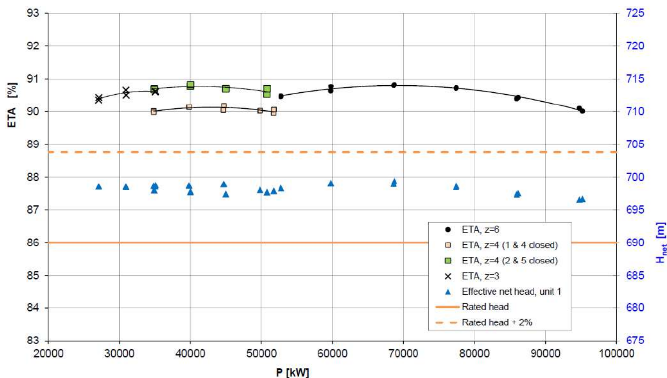
Figure 1: Results at effective net head
