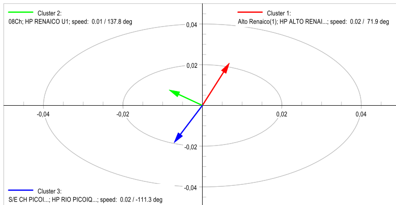
Mode 2180: Observability
