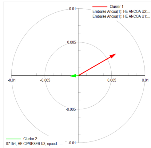
Mode 994: Observability
