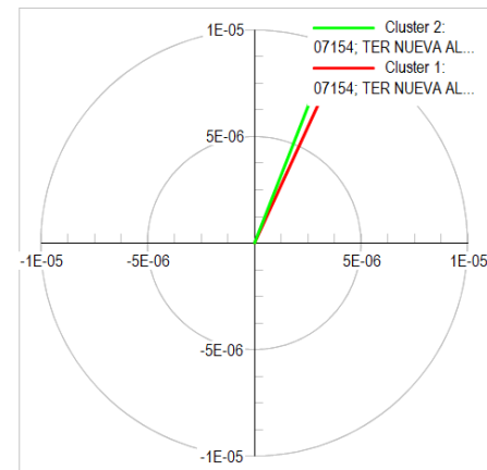
Mode 37: Observability
