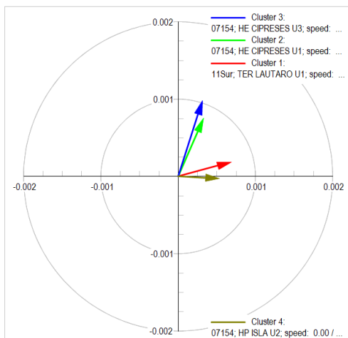
Mode 992: Observability
