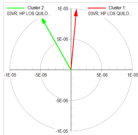
Mode 81: Observability
