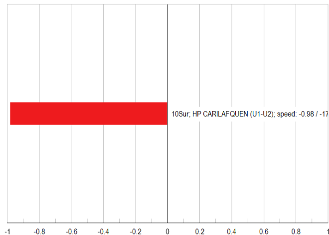
Mode 20: Participation
