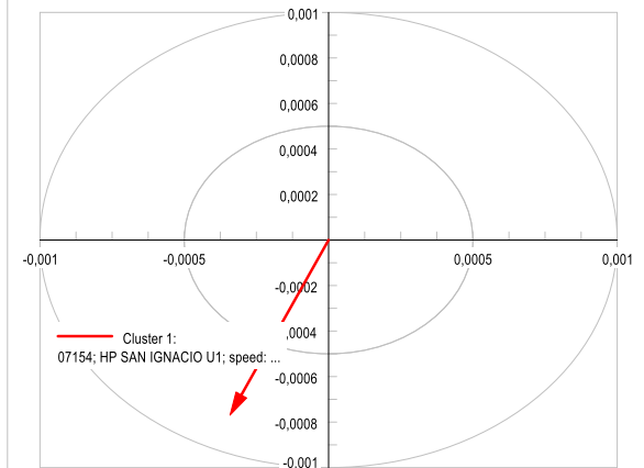
Mode 47: Observability
