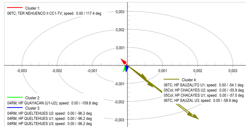
Mode 1661: Observability
