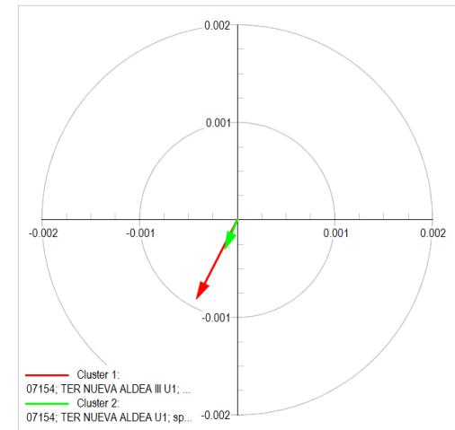
Mode 771: Observability
