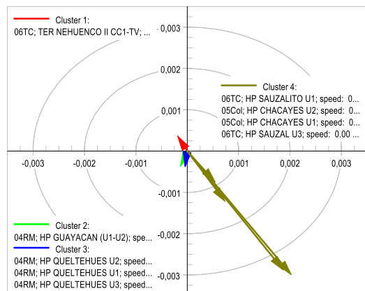
Mode 1661: Observability
