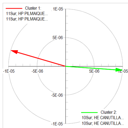
Mode 85: Observability
