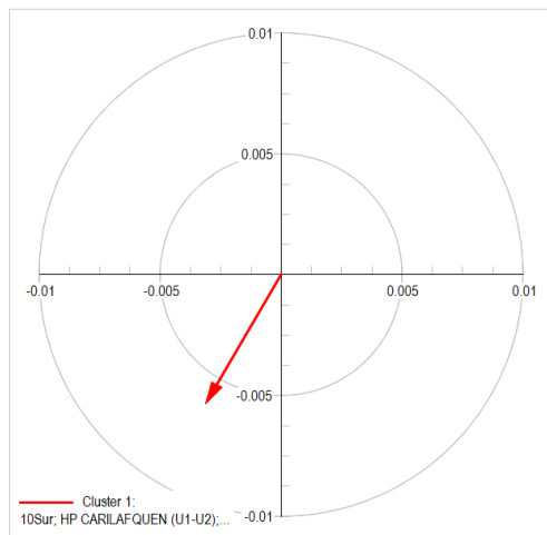
Mode 677: Observability
