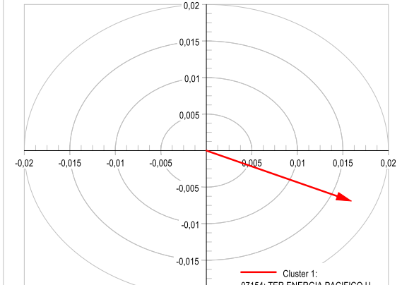
Mode 1853: Observability
