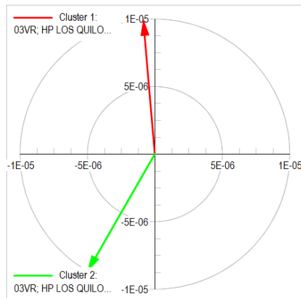
Mode 83: Observability
