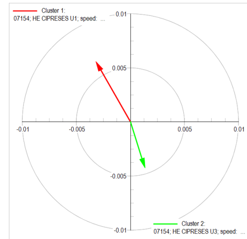
Mode 744: Observability
