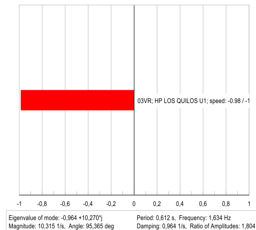
Mode 1909: Participation
